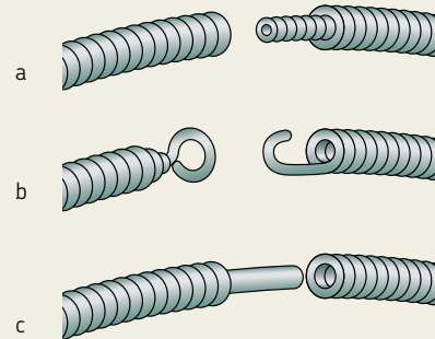
Spring connections
