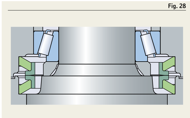
HDDF metal face seal
