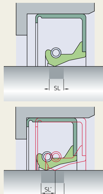
Counterface for radial shaft seals
