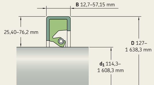
HDS nominal housing dimensions
