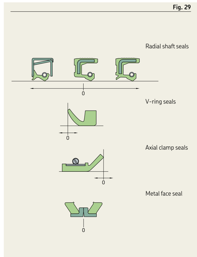
Axial movement
