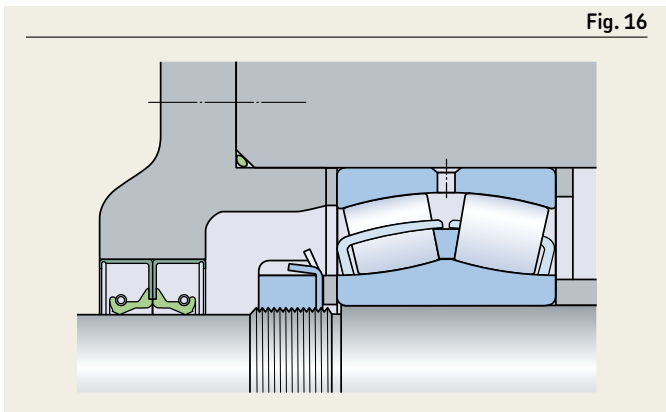
CRW1 seals
