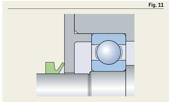
V-ring
