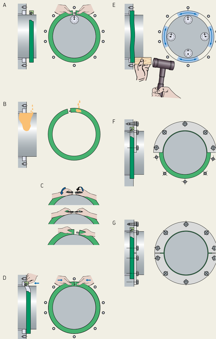
Installing an all-rubber split seal
