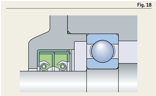
HDSD2 seal
