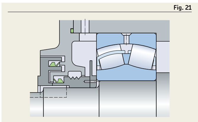
V-ring seal
